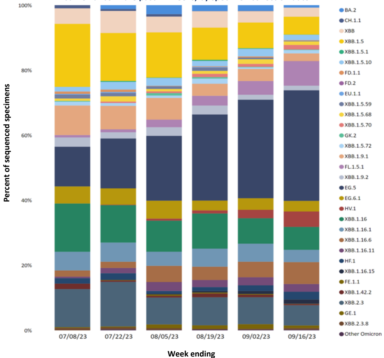
Figure 4. Variants of Concern as a percentage of all specimens sequenced for baseline surveillance in the past 12 weeks, by specimen collection date
